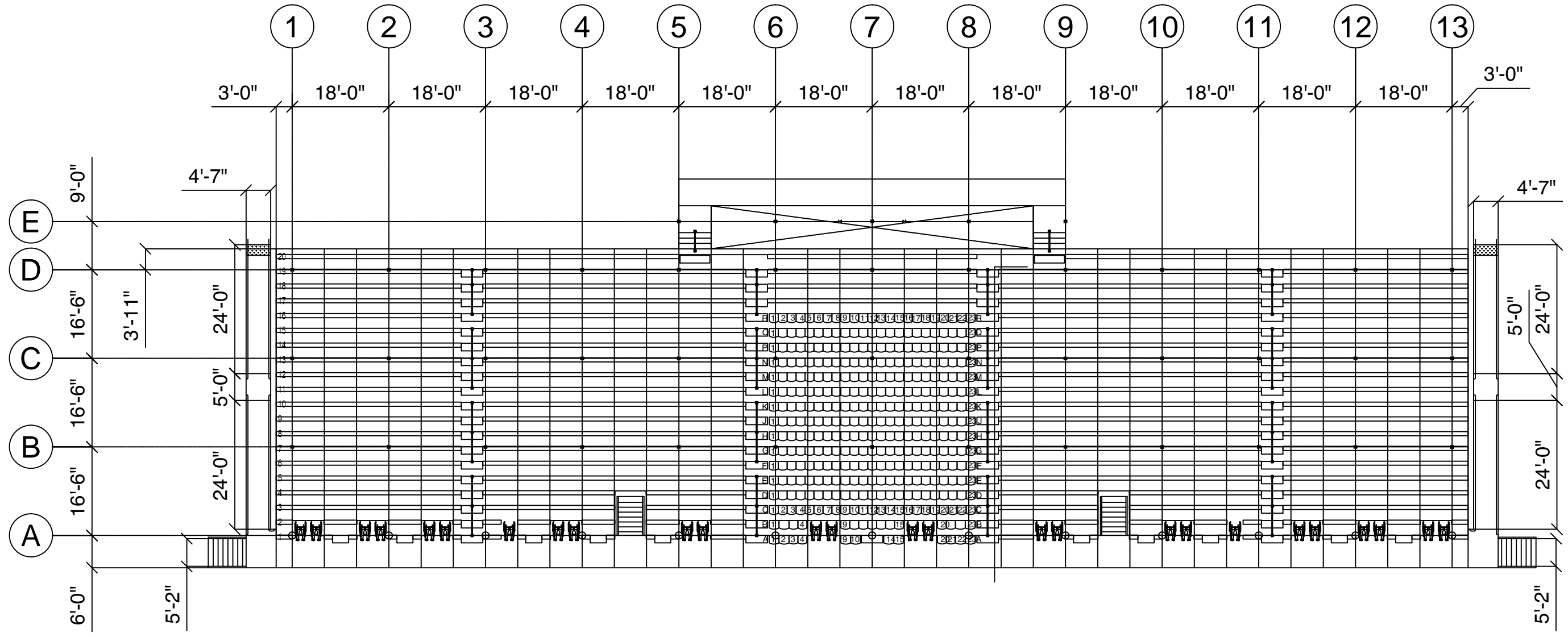
TYPICAL I-BEAM SEATING LAYOUT
