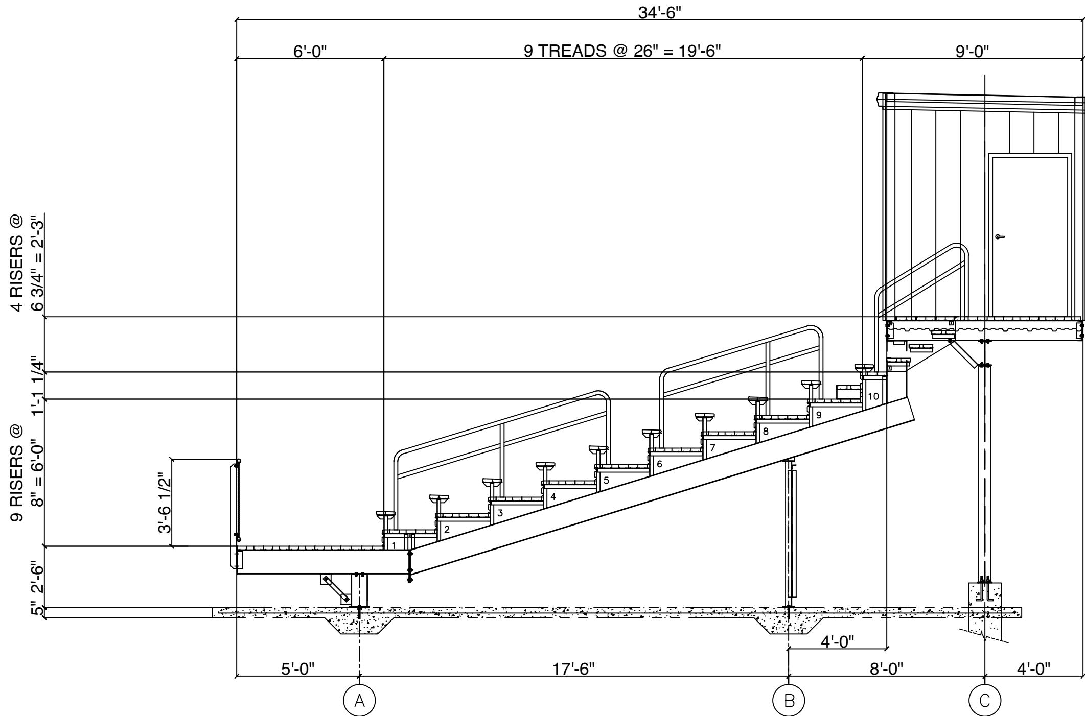
TYPICAL LEG TRUSS CROSS SECTION WITH PRESS BOX N.T.S.
