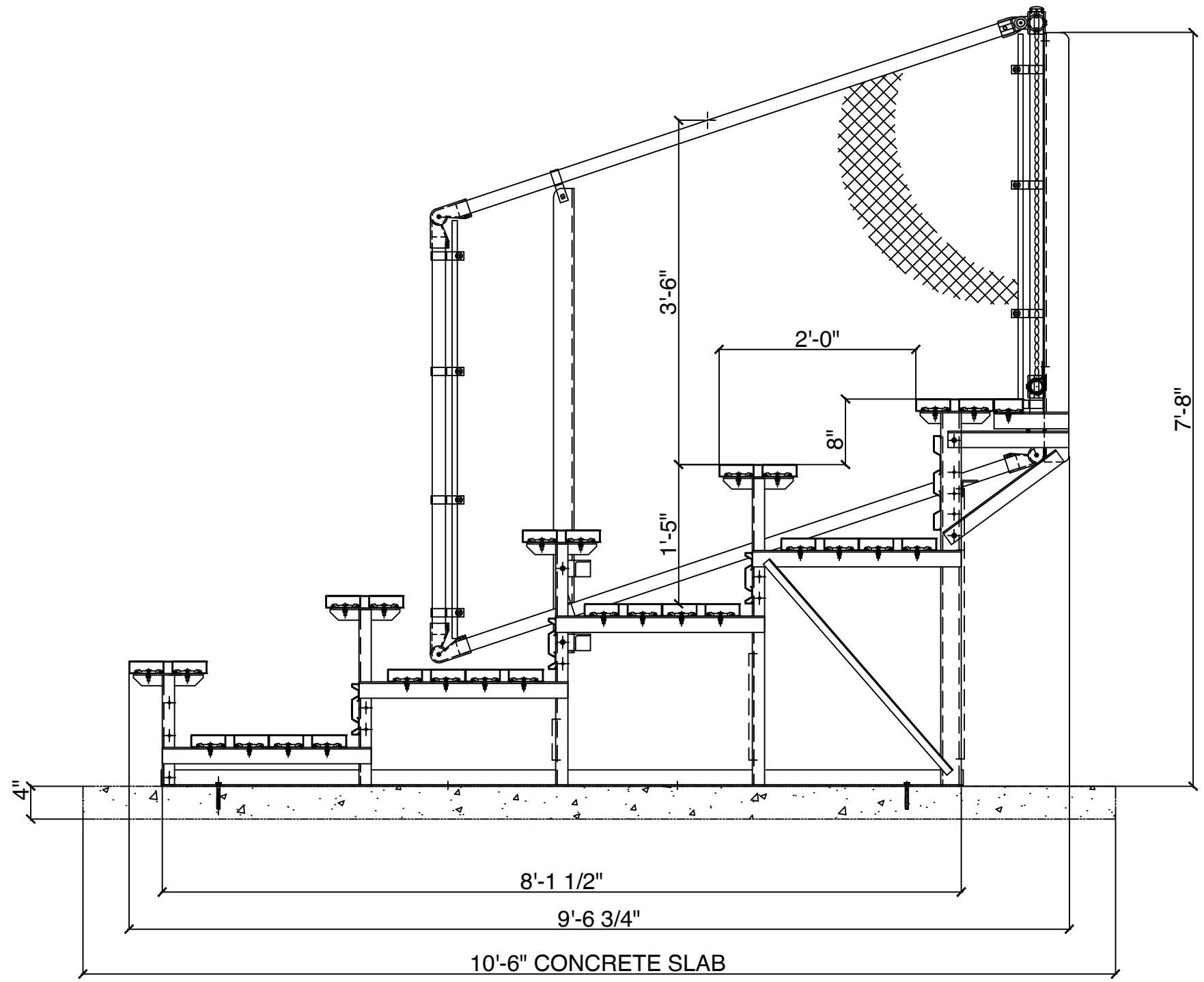
TYPICAL ANGLE FRAME CROSS SECTION 5 ROW N.T.S.
